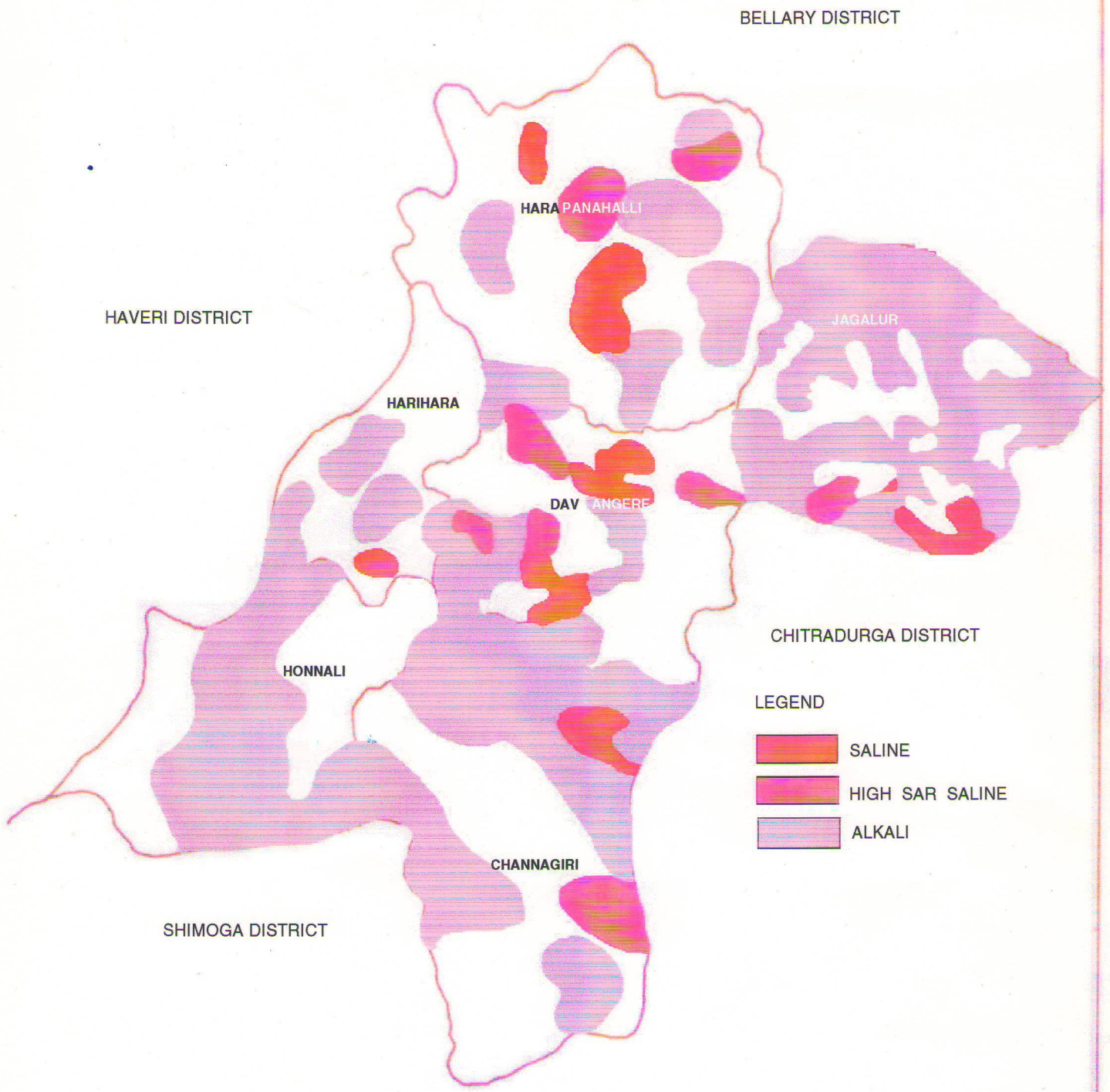
DISTRIBUTION OF POOR QUALITY GROUND WATERS IN DAVENGERE DISTRICT
